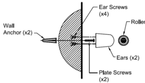
Exploded View - Side
